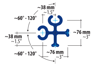
Cross connector
